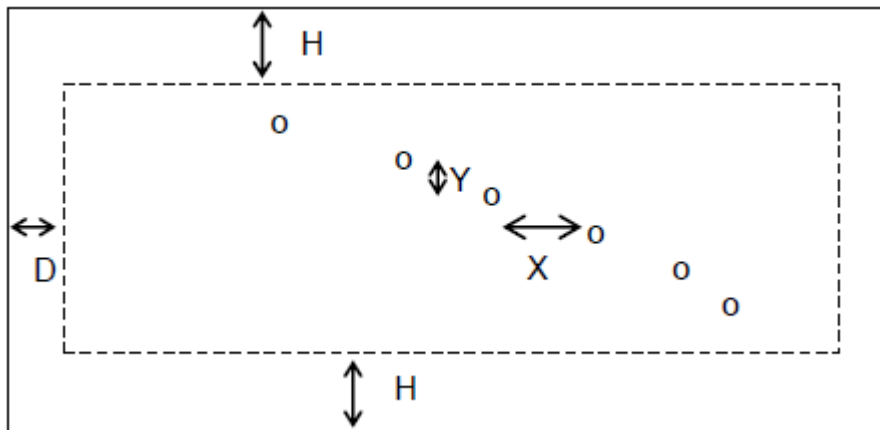
Fig. 2: Recommendations for selecting the Measurement Points on a concrete wall.
